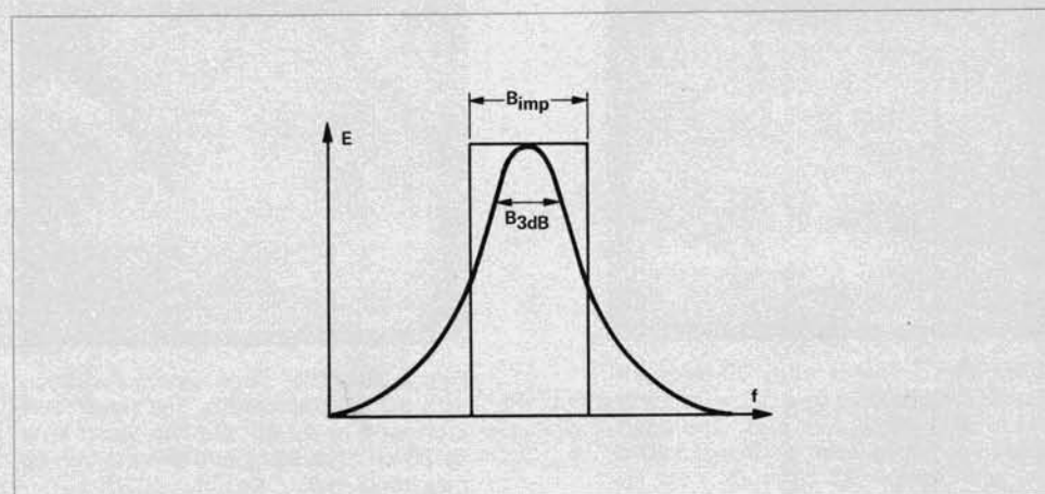
Figure 27. Equivalent B_{imp} of Gaussian filter.
