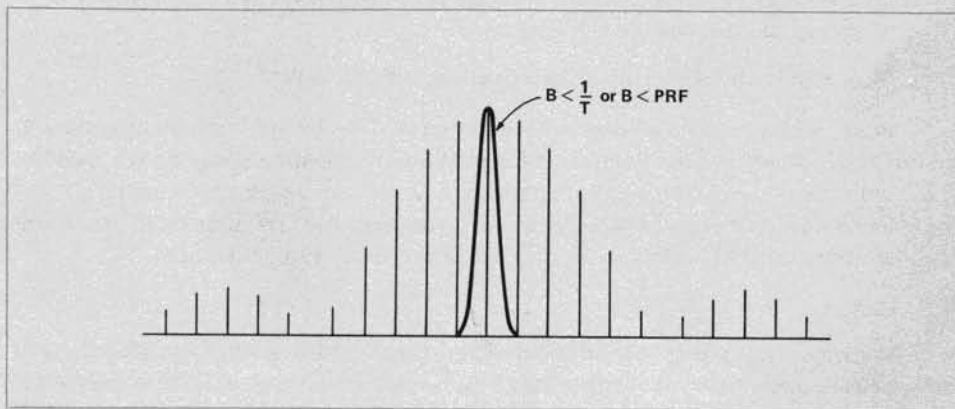
Figure 6. IF bandwidths smaller than PRF.
