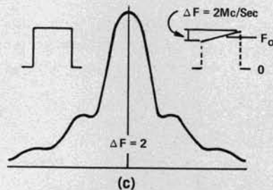
(c) Spectrum of rectangular pulse with linear FM resulting in increased sidelobe amplitude and minimas not reaching zero.
