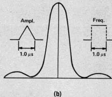
(b) Triangular pulse spectrum without FM during pulse. Effective pulse width is shorter than (a) causing minimas to occur at wider intervals of frequency.
