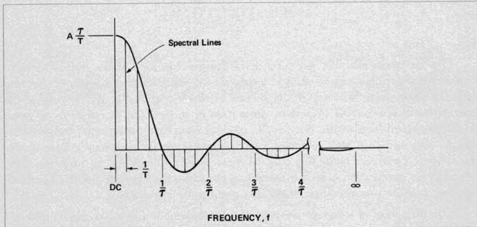
Figure 2. Spectrum of a perfectly rectangular pulse. Amplitudes and phases of an infinite number of harmonics are plotted, resulting in smooth envelope as shown.
