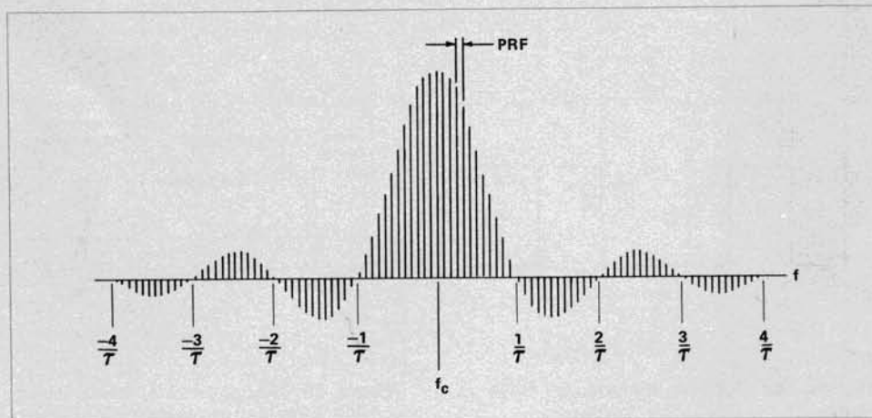
Figure 3. Resultant spectrum of a carrier amplitude modulated with a rectangular pulse.
