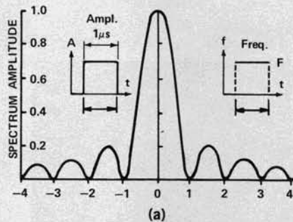
(a) Spectrum of rectangular pulse without AM or FM occurring during pulse. Shape is that of \frac{\sin \omega \frac{\tau}{2}}{\omega \frac{\tau}{2}} function.
