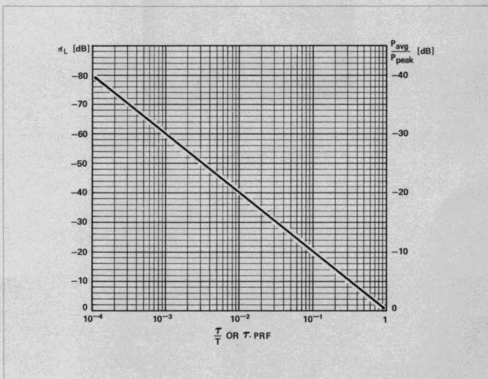
Figure 14. Pulse desensitization \alpha_L (line spectrum).
