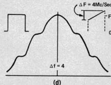
(d) Same pulse spectrum as (c) with more severe FM.
