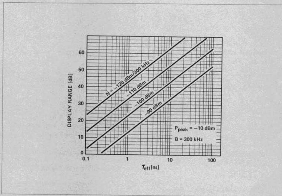
Figure 29. Display range vs. sensitivity.
