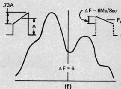
(f) More severe case of FM and AM occurring during pulse.
