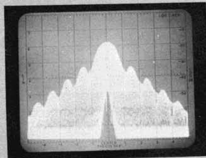
Figure 23. Same signal with B = 3 kHz.
